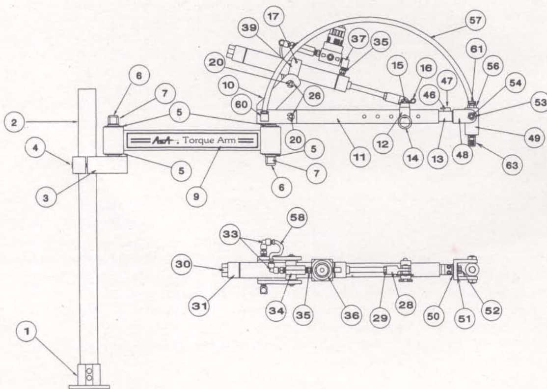
STD-15110-AC—Air Cylinder Ast Torque Arm
