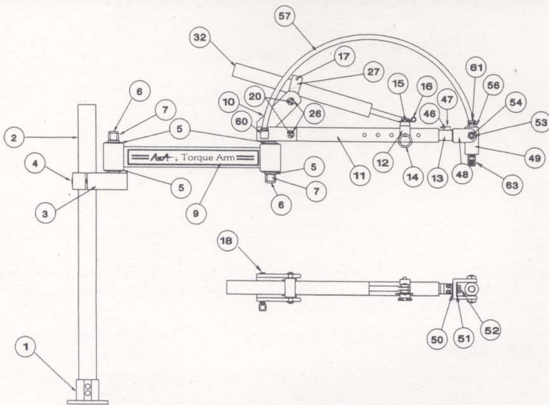
STD-03110-OC—Oil cylinder Ast Torque Arm
